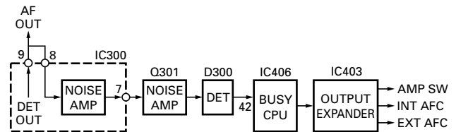
Fig. 5 Squelch circuit
