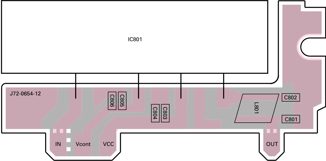
FINAL UNIT (X45-3590-10) Component side view : K3,K6
