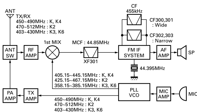
Fig. 1 Frequency configuration
