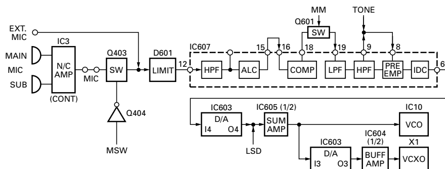
Fig. 6 Microphoen circuit
